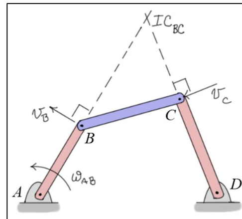
General Configuration
